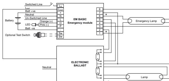
Single lamp high frequency electronic ballast
