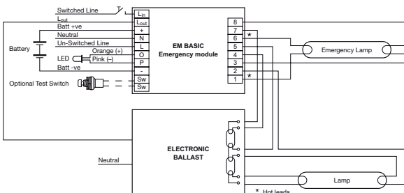
Twin series switch start circuit with conventional control gear
