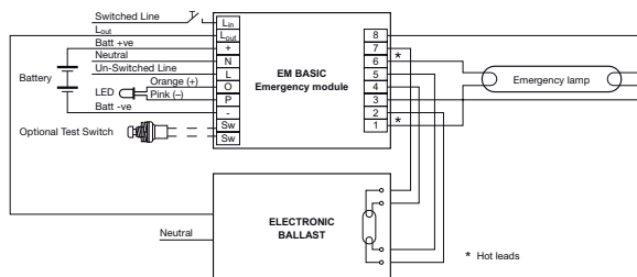
Single lamp high frequency electronic ballast
