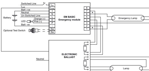
Twin lamp high frequency electronic ballast (8 lamp lead connections)
